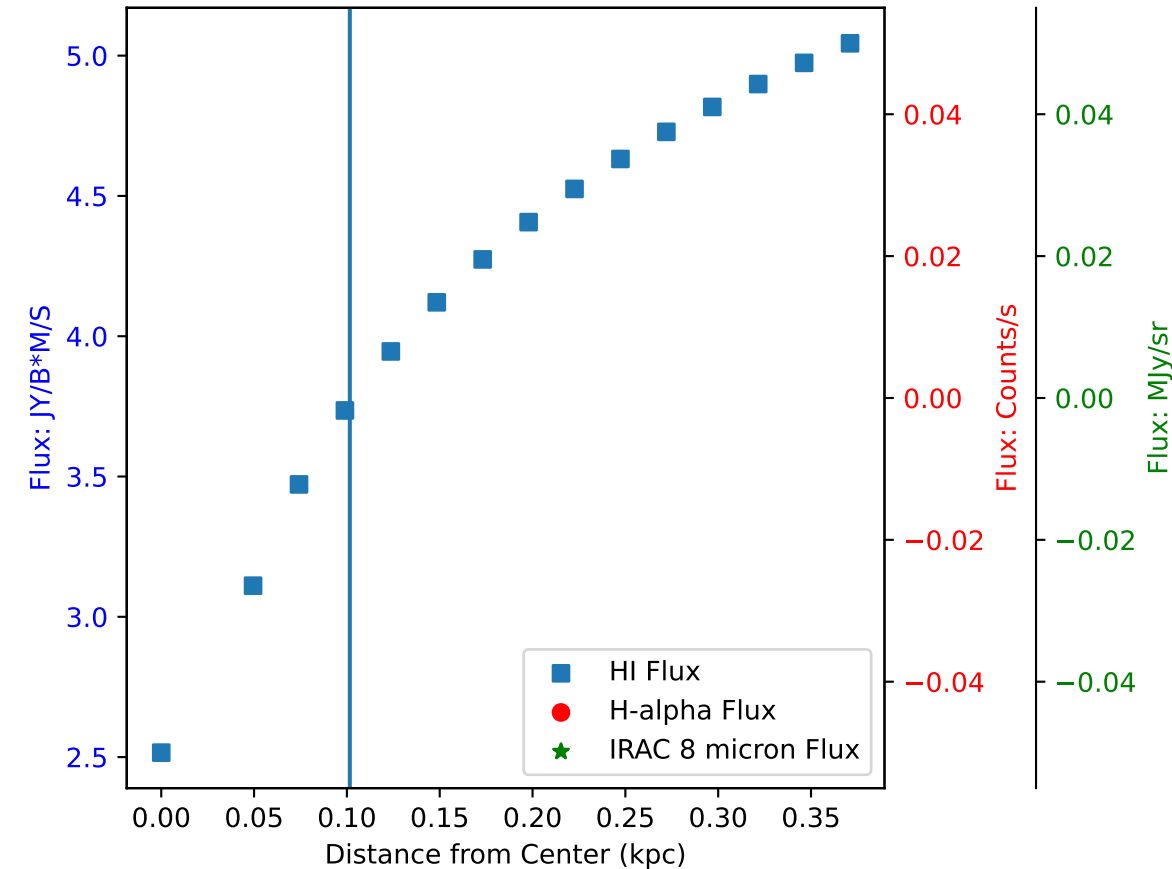
Flux of HI vs. H-alpha in Galaxy: DDO 50 - Region 8
