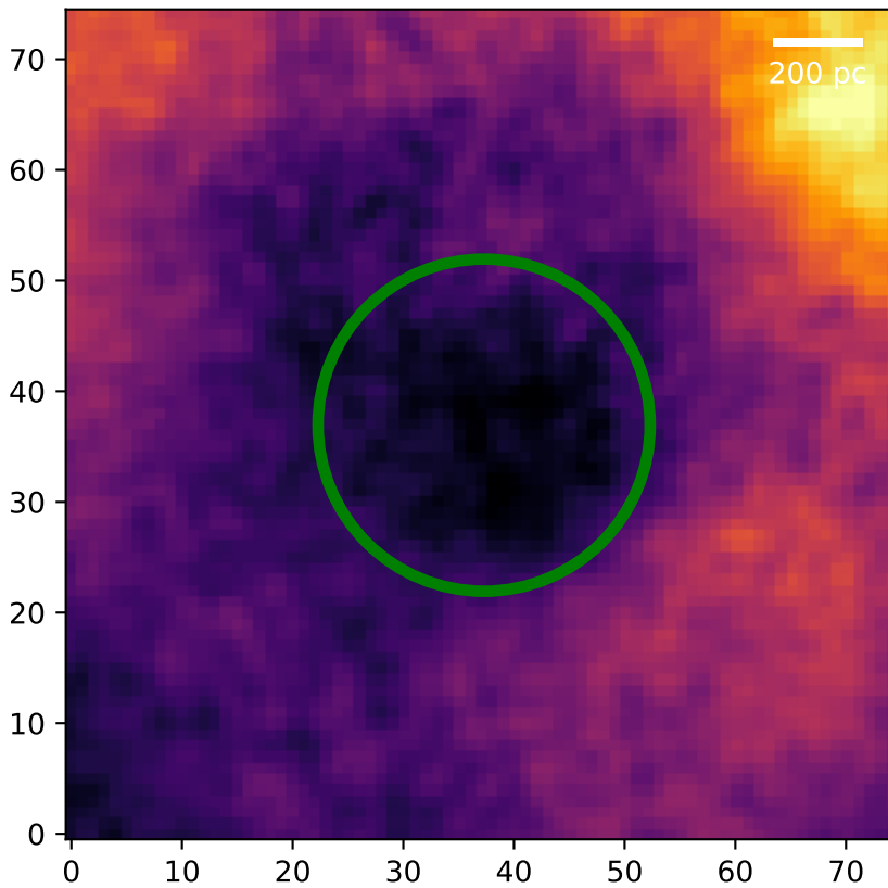
Region: 34 HI - Type 1
