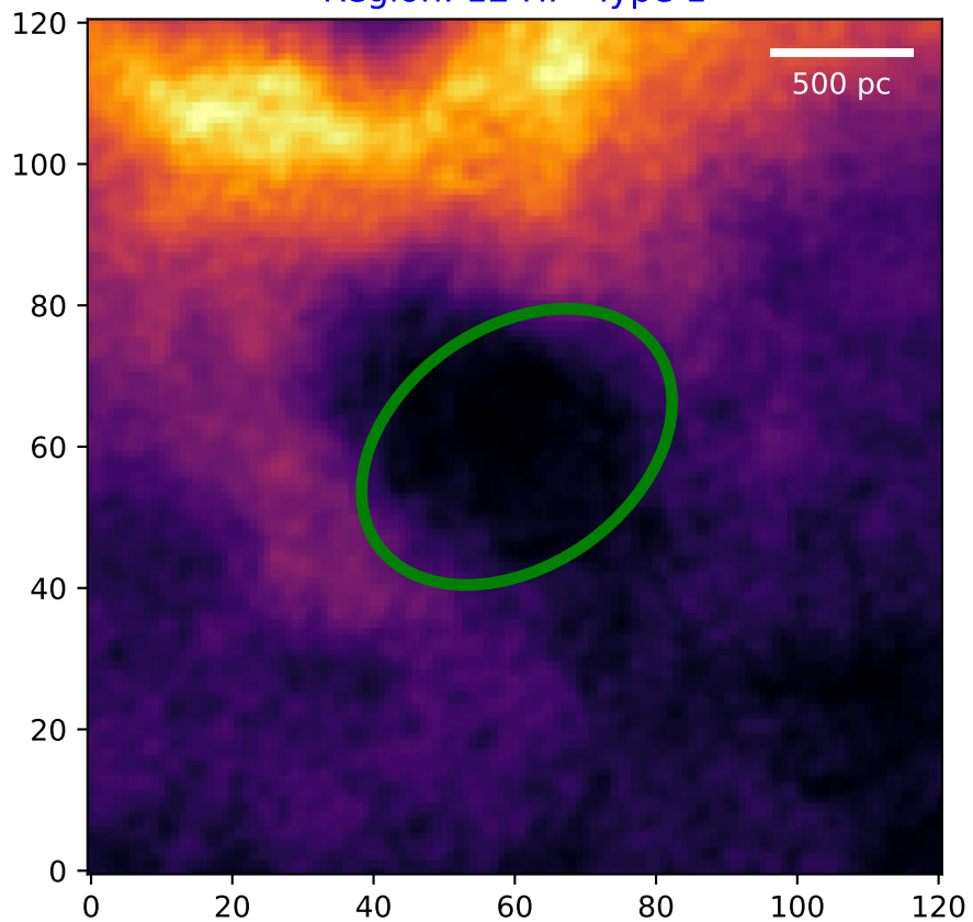
Region: 12 HI - Type 1
