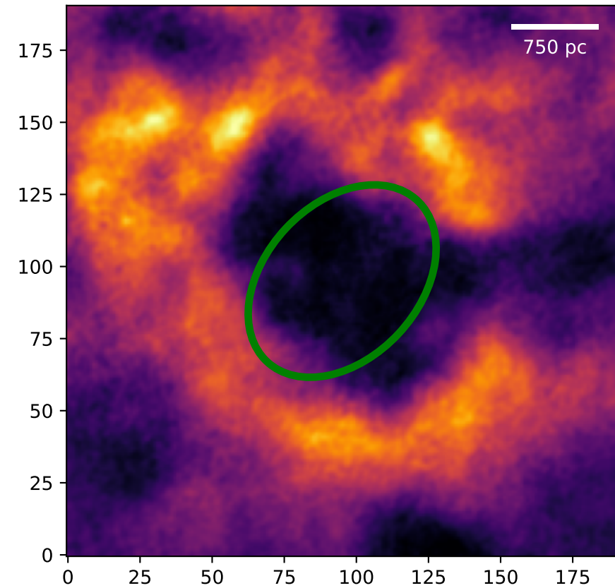
Region: 18 HI - Type 1
