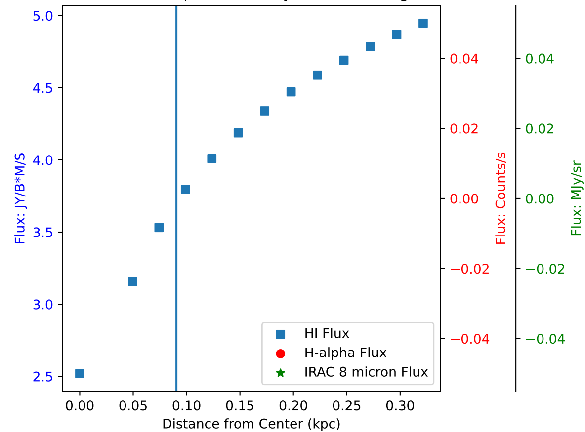
Flux of HI vs. H-alpha in Galaxy: DDO 50 - Region 25
