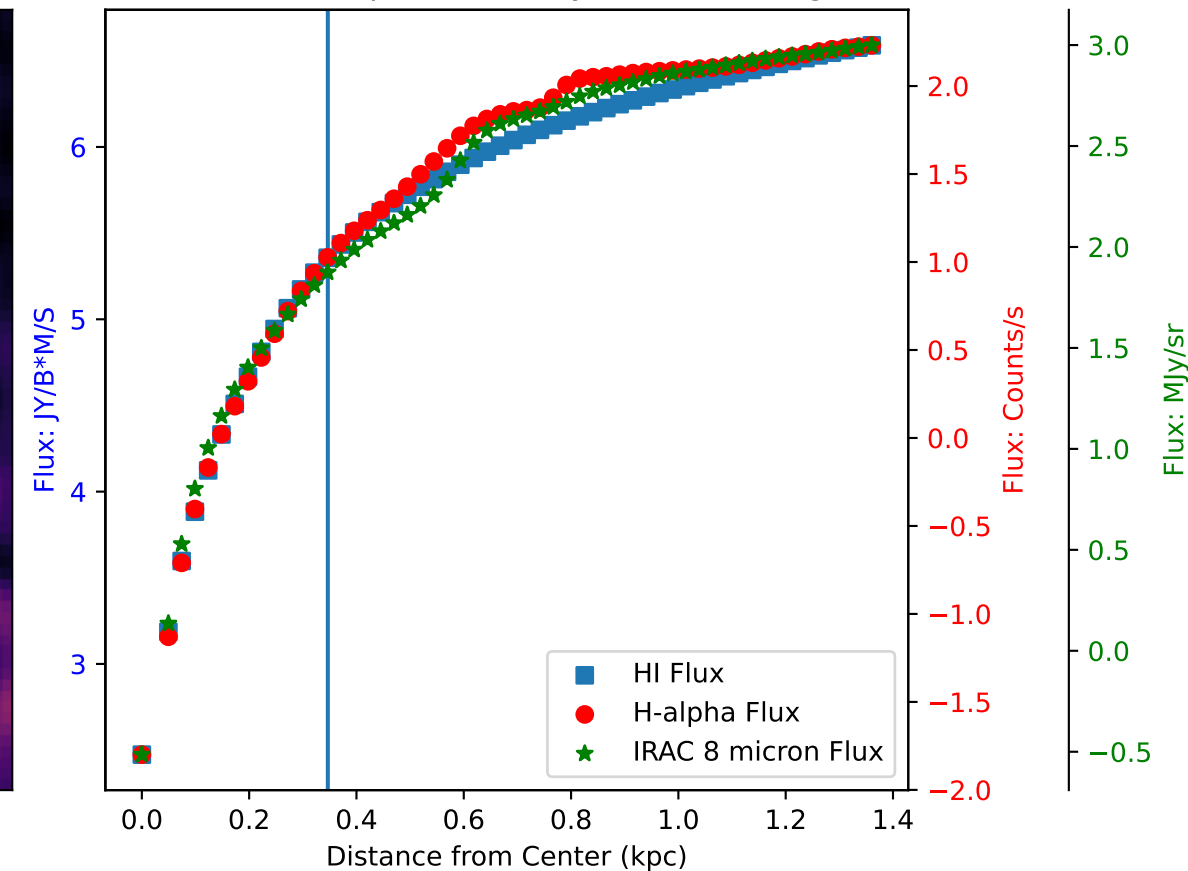
Flux of HI vs. H-alpha in Galaxy: DDO 50 - Region 16
