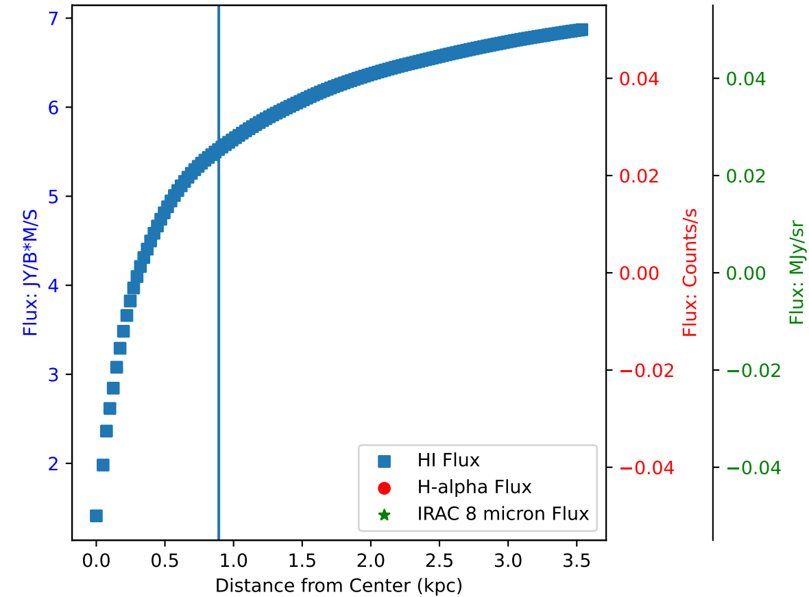
Flux of HI vs. H-alpha in Galaxy: DDO 50 - Region 40
