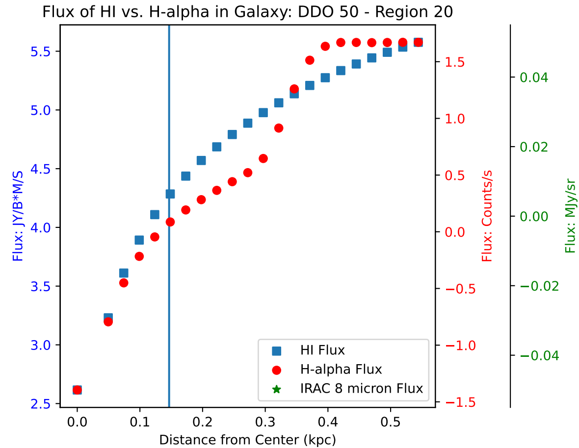
IRAC 8 micron - Classification: No Emission
