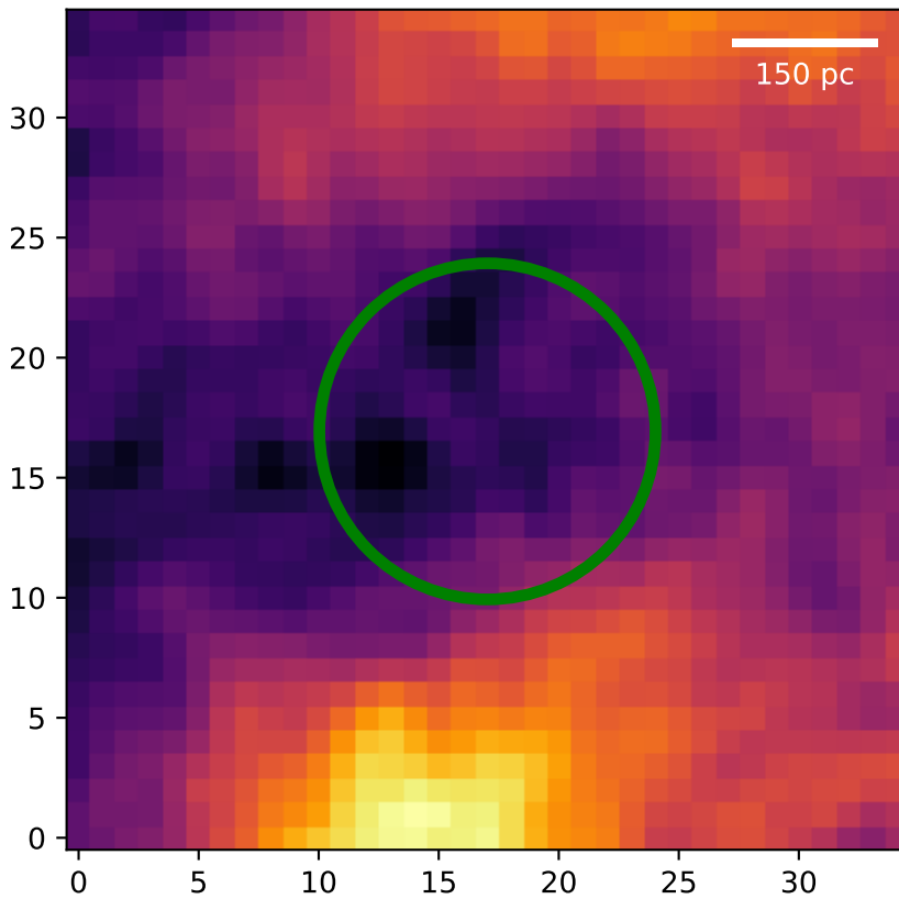
Region: 31 HI - Type 3
