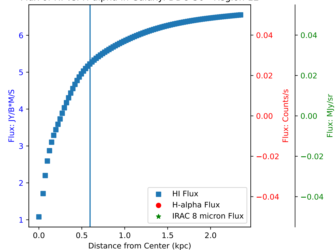
Flux of HI vs. H-alpha in Galaxy: DDO 50 - Region 12
