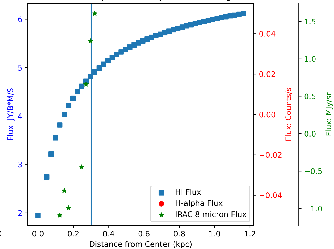
Flux of HI vs. H-alpha in Galaxy: DDO 50 - Region 27
