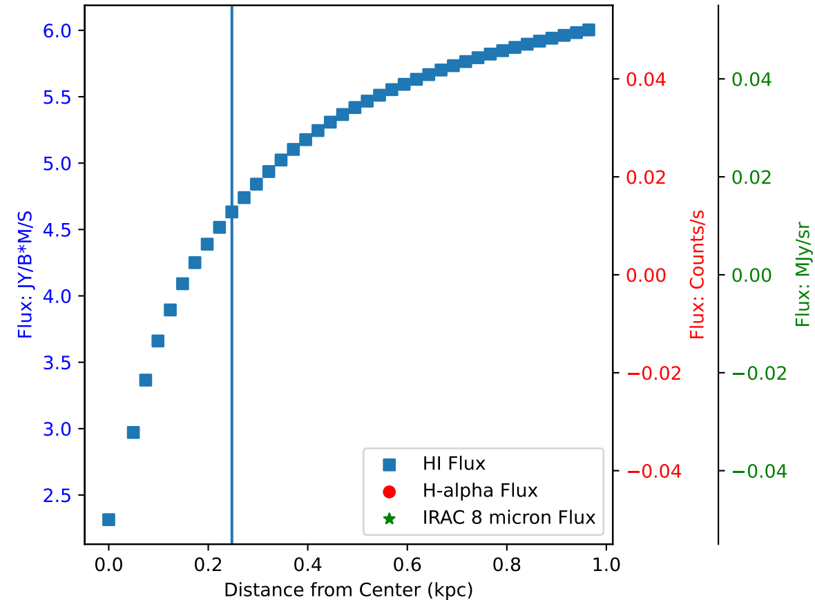
Flux of HI vs. H-alpha in Galaxy: DDO 50 - Region 26
