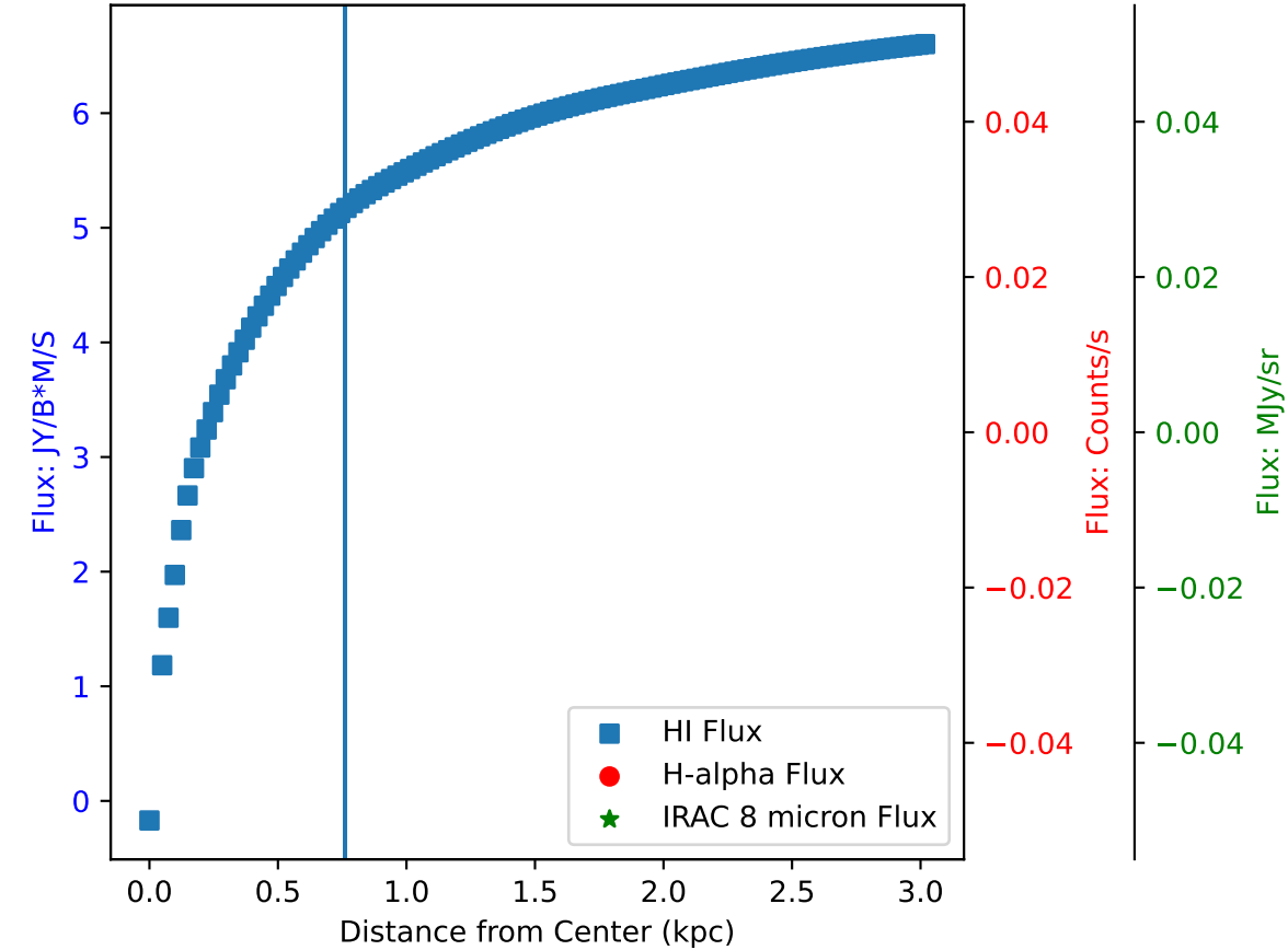
Flux of HI vs. H-alpha in Galaxy: DDO 50 - Region 1
